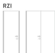
Ceiling-height frame without head and transom up to a clear ceiling height of 2,600 mm (single leaf, double leaf)
