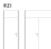
Ceiling-height frame without head and transom, with top panel up to a clear ceiling height of 2,600 mm (single leaf, double leaf)
