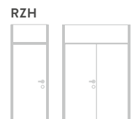
Ceiling-height frame without head, with transom and fanlight up to a ceiling height of 2,600 mm (single leaf, double leaf)
