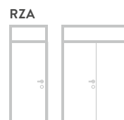
Ceiling height frame with head, transom and fanlight up to a clear frame height of 2,520 mm (single leaf, double leaf)
